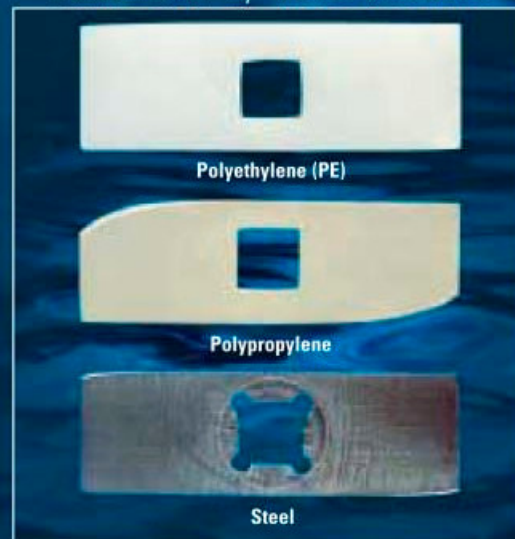
Samples of material after 24 hours in a mixture of quartz sand and water (ratio 3:2) at 1200 rpm
